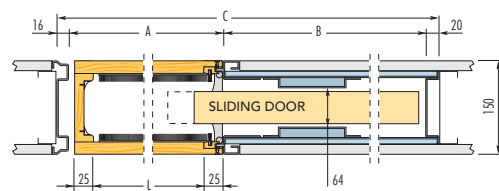
HEAD SECTION AND JAMB POST COMPLETE WITH BRUSH STRIP AND SEALS
