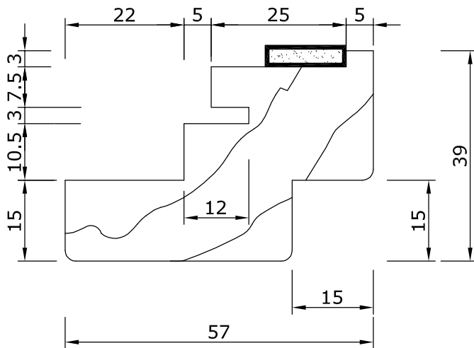
Vertical post - counterframe side nr.1 left piece + nr.1 right piece Length 2098 mm
