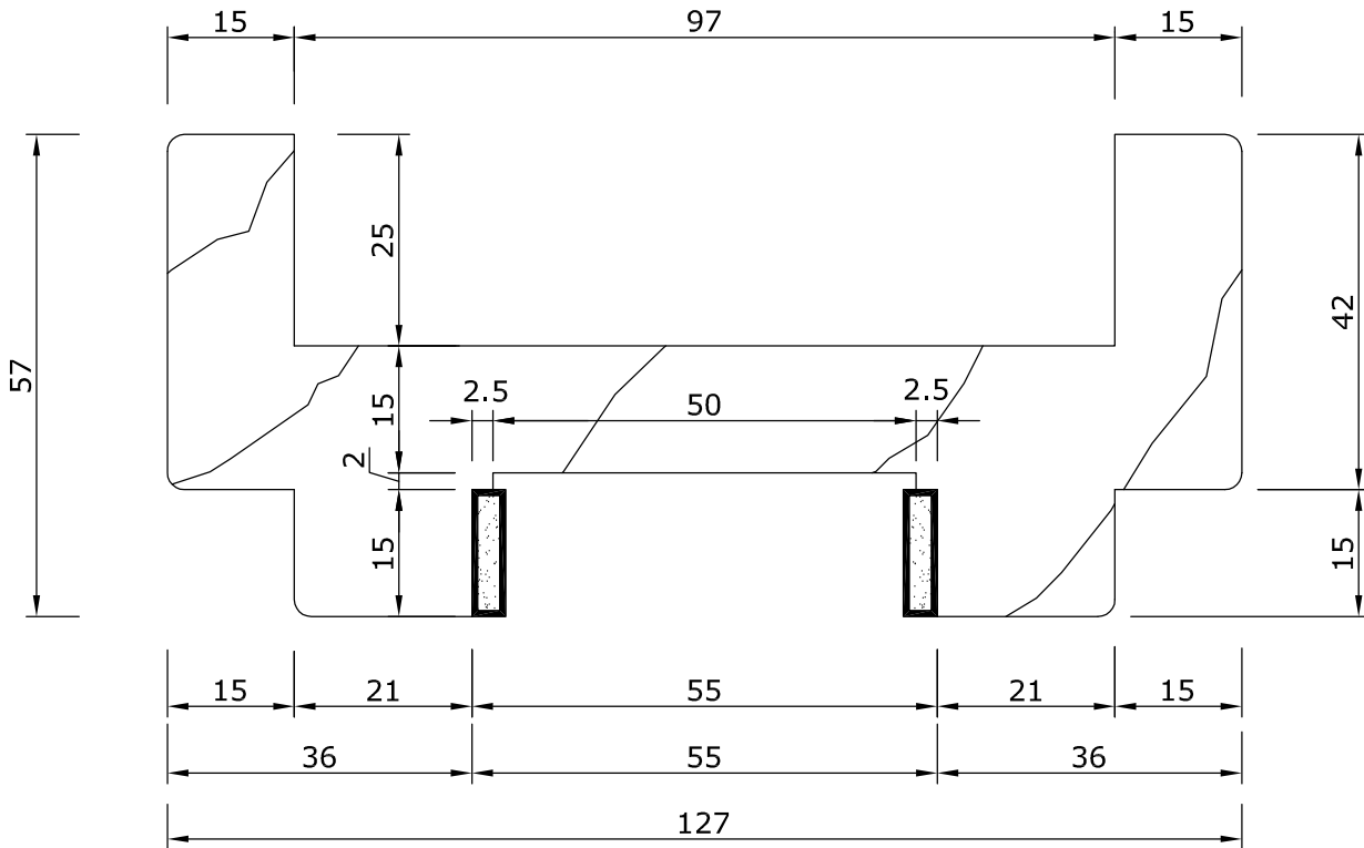
Front post 1 piece Length 2098 mm
